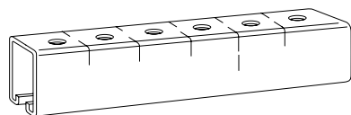
For heavier load requirements. Connection by means of continuous slot or \frac{9}{16} " holes on 1\frac{1}{2} " centers.
