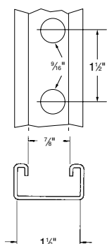
Connection by means of continuous slot or \frac{9}{16} " holes on 1\frac{1}{2} " centers.
